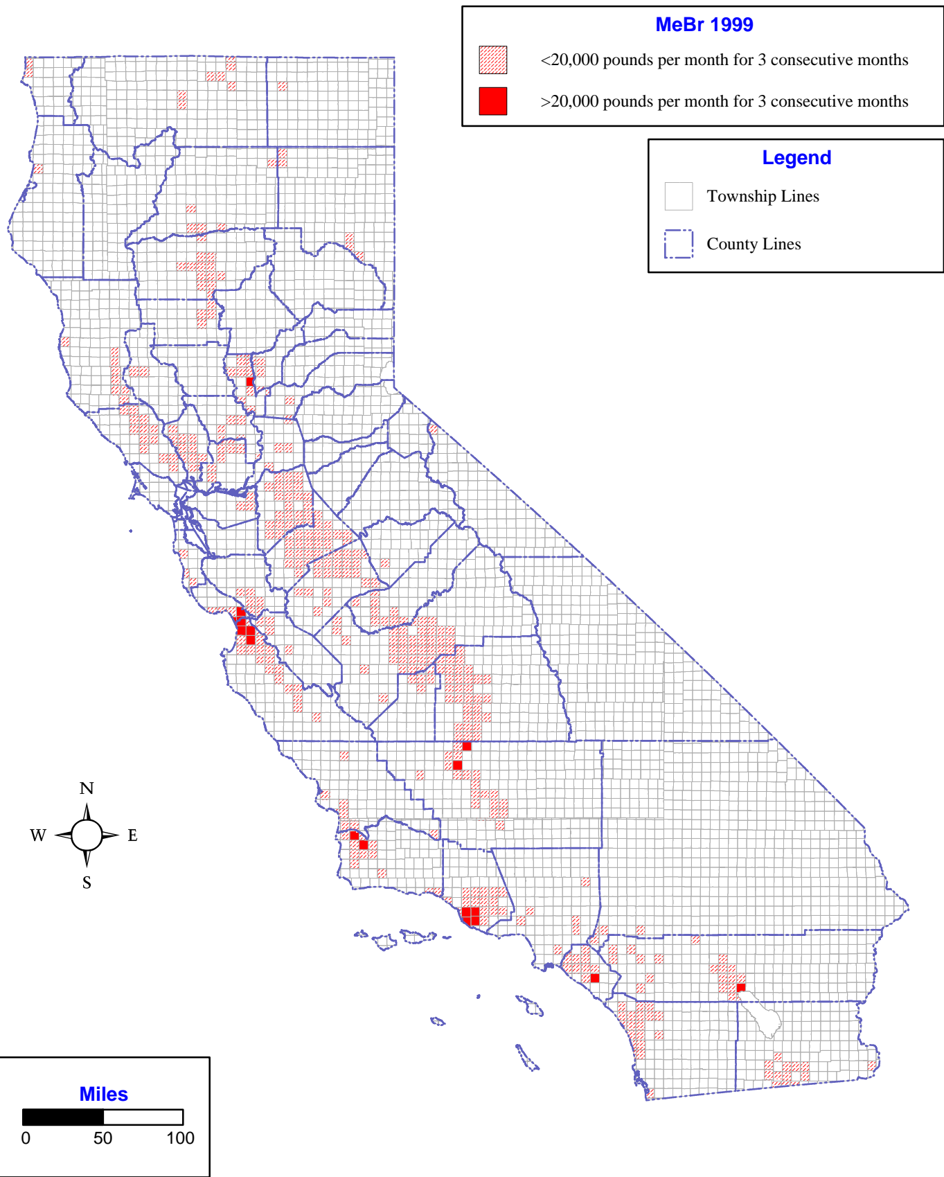
Fig 13. Methyl Bromide Use in California (1999)
