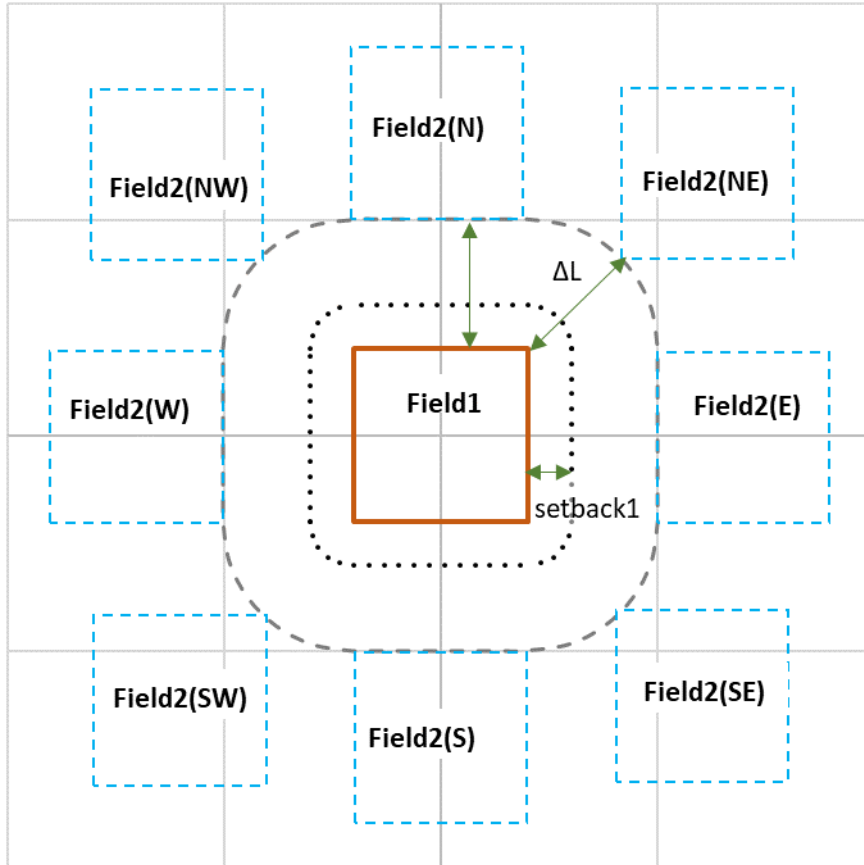
Figure 6. Simulation domain for multiple applications, showing the main source “Field1” and the eight potential locations of the 2 nd source “Field2” with a distance of \Delta L from “Field1”. Black dots represent receptors at the required setback distance for “Field1”.
