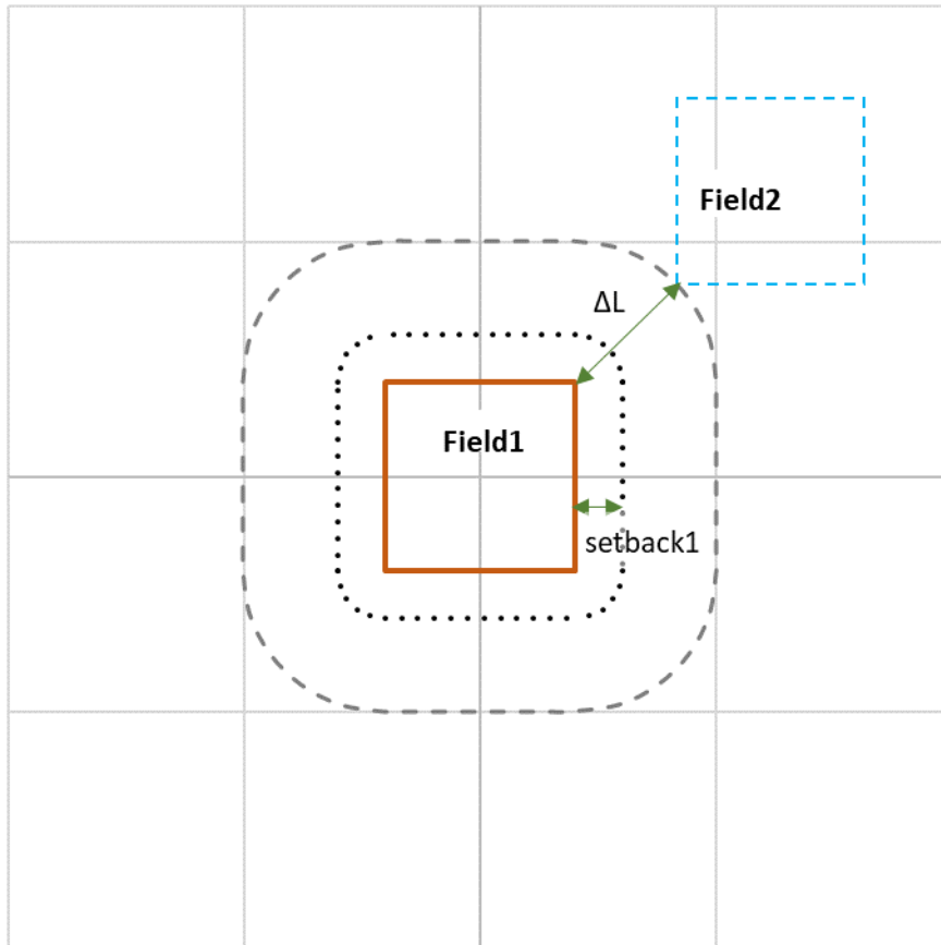
Figure 5. Definition of the distance between two fields. The dashed line delineates a perimeter with the same distance \Delta L . Black dots represent receptors at the required setback distance for “Field1”.
