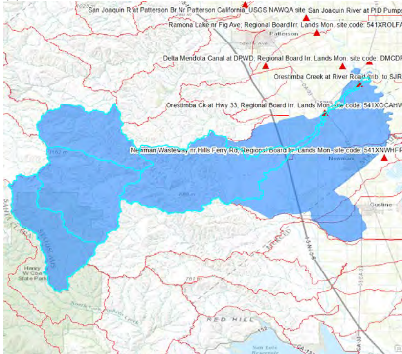
Figure 3. Actual drainage areas (blue) and drainage areas defined by HUC12 (highlighted): (a) Slisal Slough @ Hartnell Rd (HUC12=180600051509), and (b) Orestimba Creek @ River Rd (HUC12=180400020101-0104)
