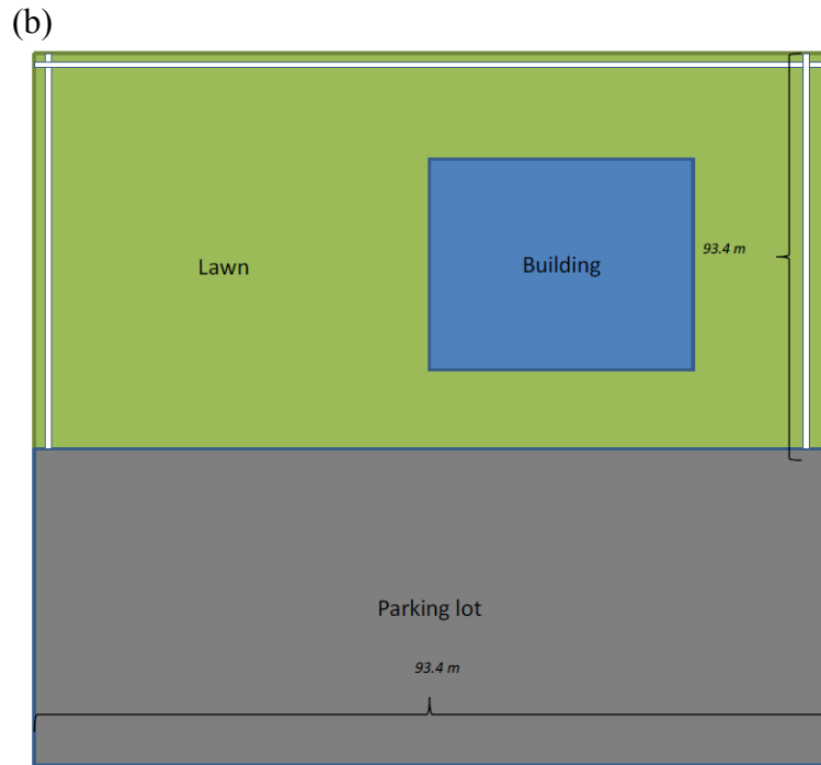
Figure 6. (a) A standard commercial/industrial watershed and (b) landscape design (the lot size: 8725 m 2 ; the building size: 1000 m 2 ), taken from USEPA effects determination for acephate (USEPA, 2011), Appendix L, figure 2. The length of the sidewalk measured in the figure should be 46.7 m (labeled as 93.4 m in the USEPA report)
