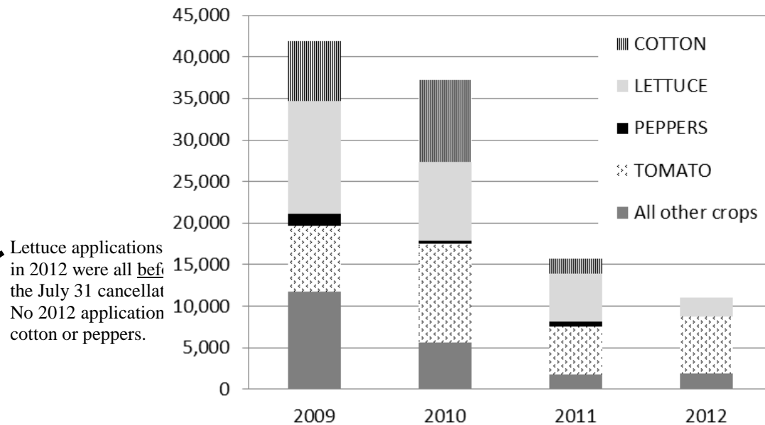
Figure 2. Endosulfan reported use within California, by crop, 2009-2012.
