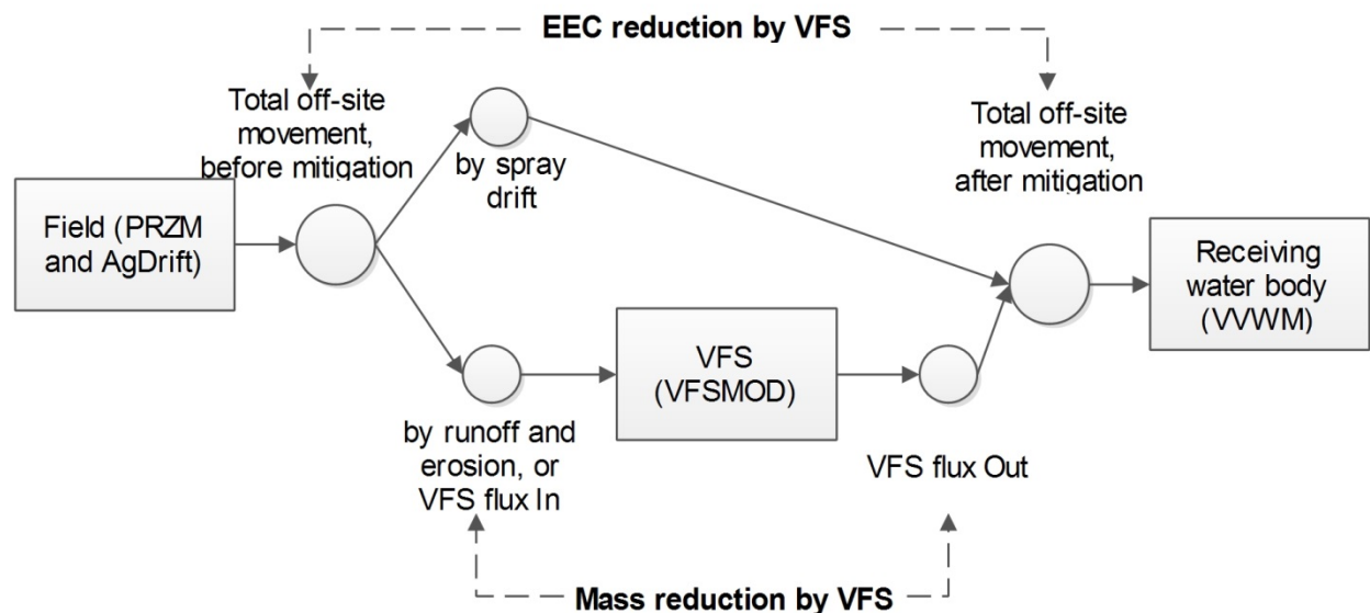
Figure 4. Diagram of the mitigation effects by vegetative buffer strip (VFS) in terms of mass reduction and EEC reduction
